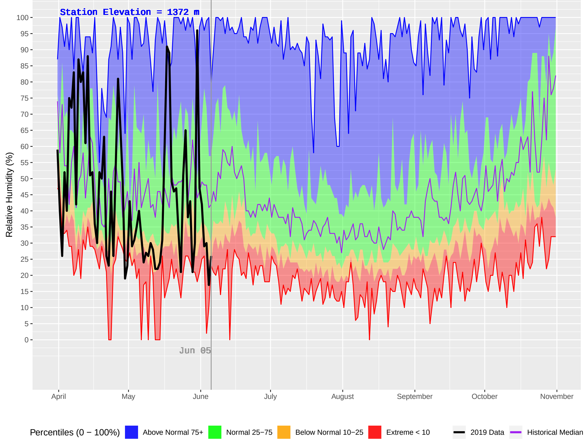
CHERRY LAKE (791) : Historical (1989–2018) and Current (2019) Daily Relative Humidity
