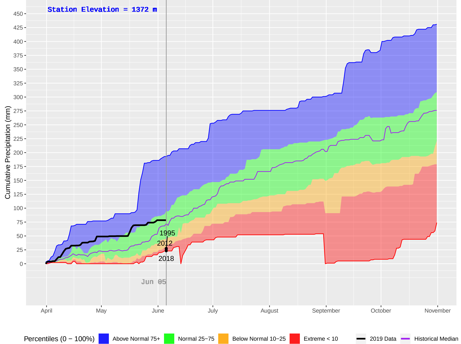
CHERRY LAKE (791) : Historical (1989–2018), Current (2019) Daily Cumulative Precipitation
