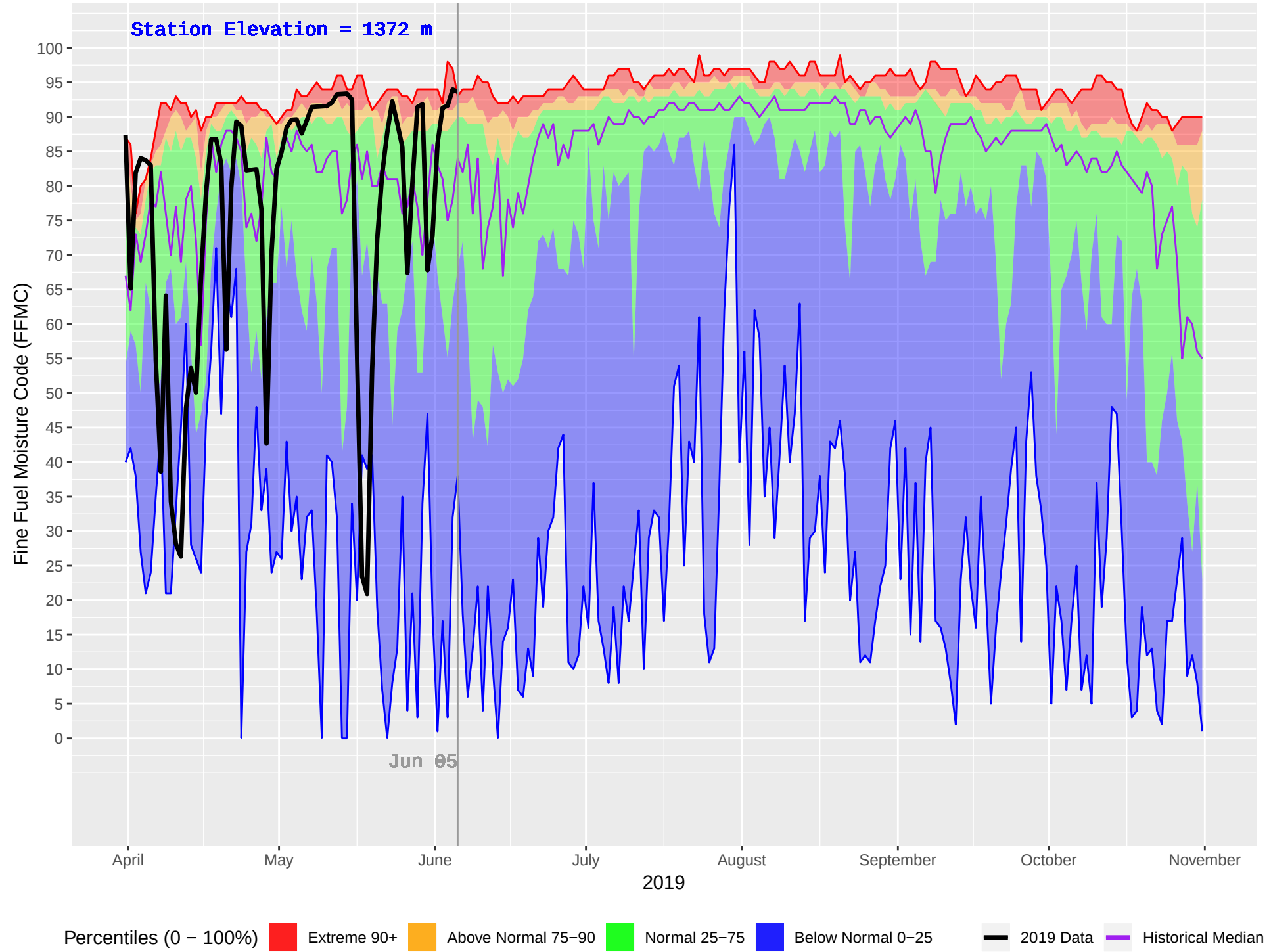
CHERRY LAKE (791) : Historical (1989–2018) and Current (2019) Daily Fine Fuel Moisture Code (FFMC)
