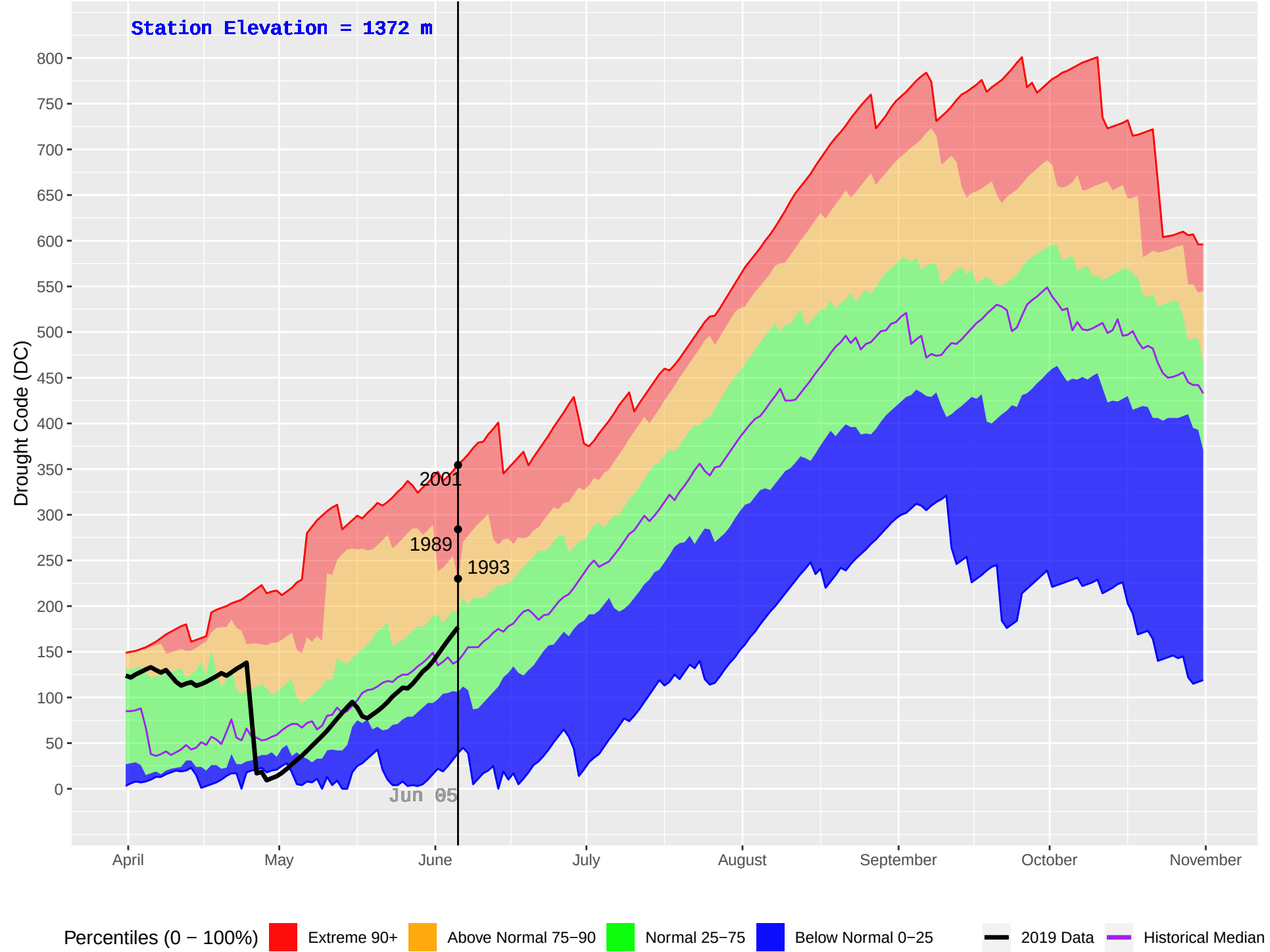
CHERRY LAKE (791) : Historical (1989–2018) and Current (2019) Daily Drought Code (DC)
