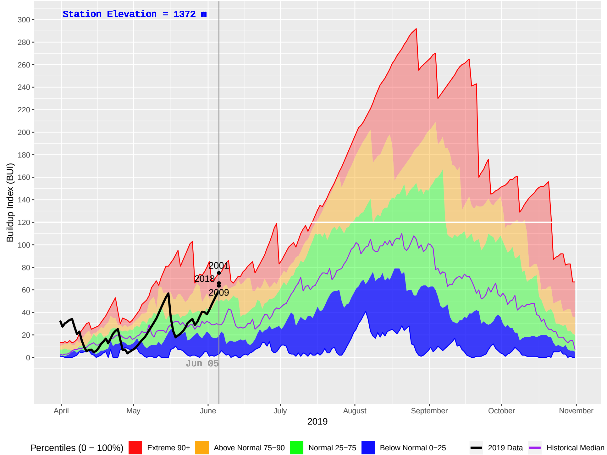
CHERRY LAKE (791) : Historical (1989–2018), Current (2019) Daily Buildup Index (BUI)
