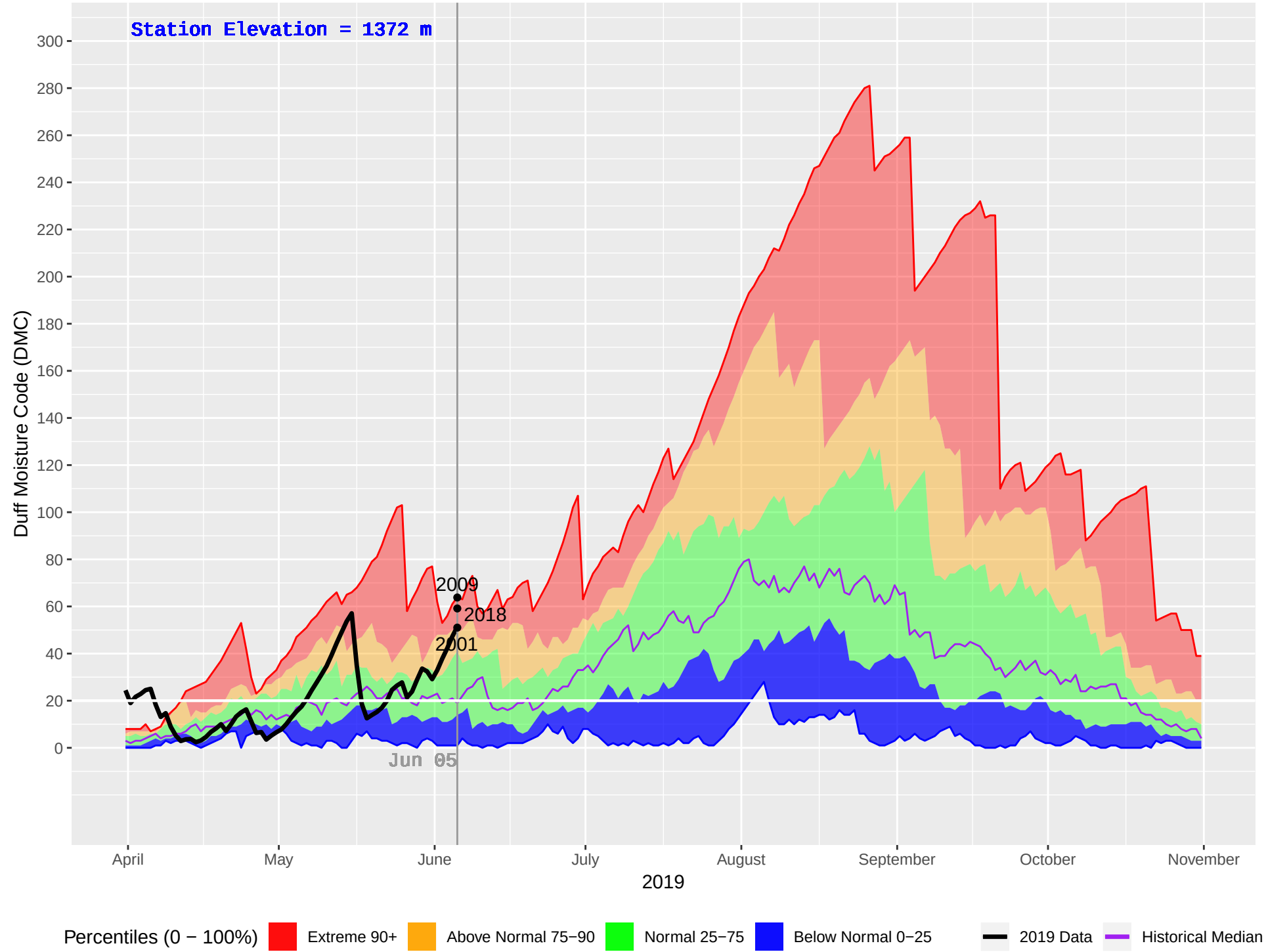
CHERRY LAKE (791) : Historical (1989–2018), Current (2019) Daily Duff Moisture Code (DMC)
